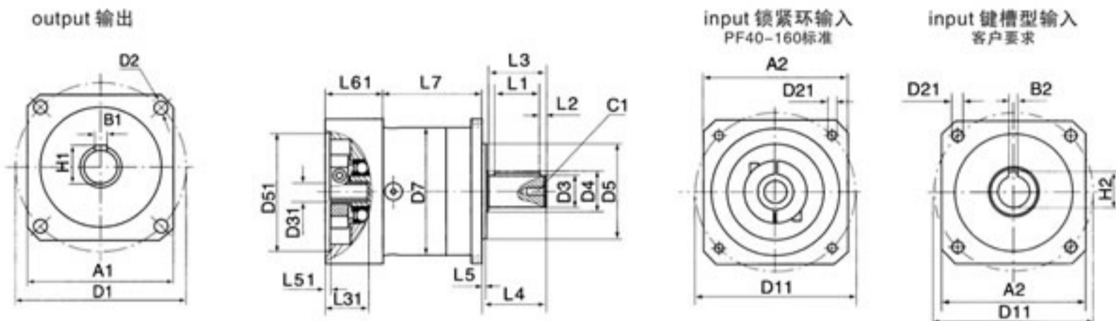
PF40-PF215-OP2 motor mounting dimensions PF40-PF215-OP2 电机联接型式外形安装尺寸
