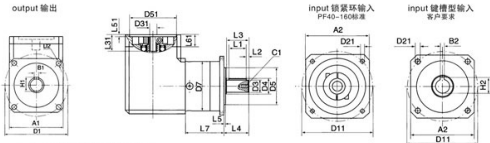
WPF40-PF215-OP2 motor mounting dimensions WPF40-WPF215-OP2 电机联接型式外形安装尺寸
